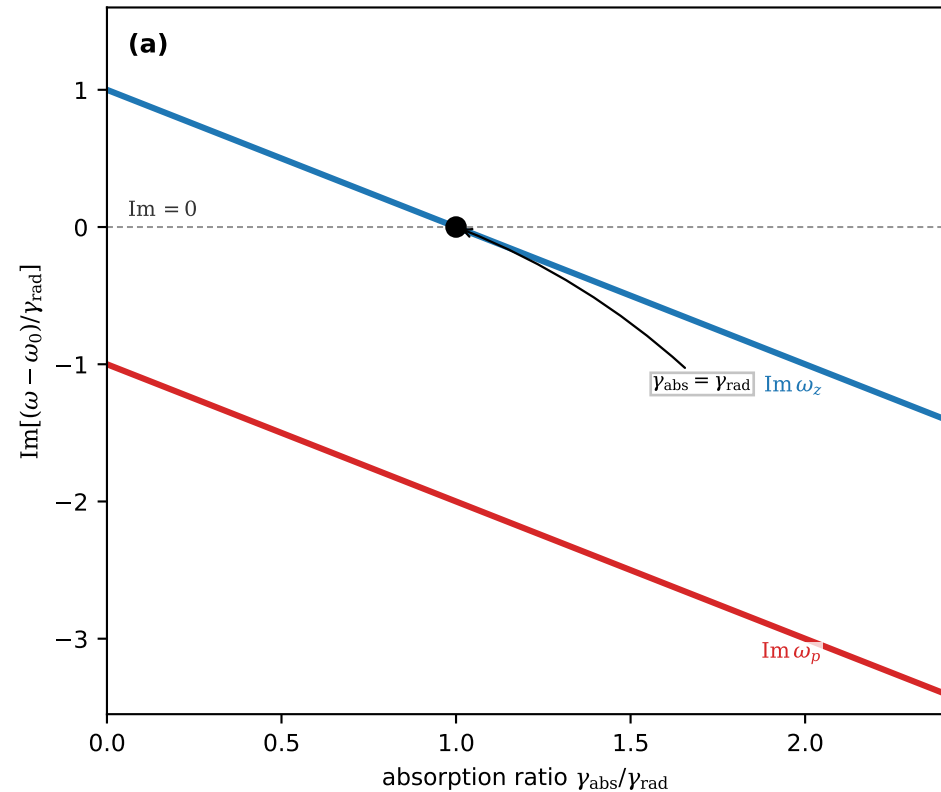
Pole and zero imaginary parts vs absorption ratio
