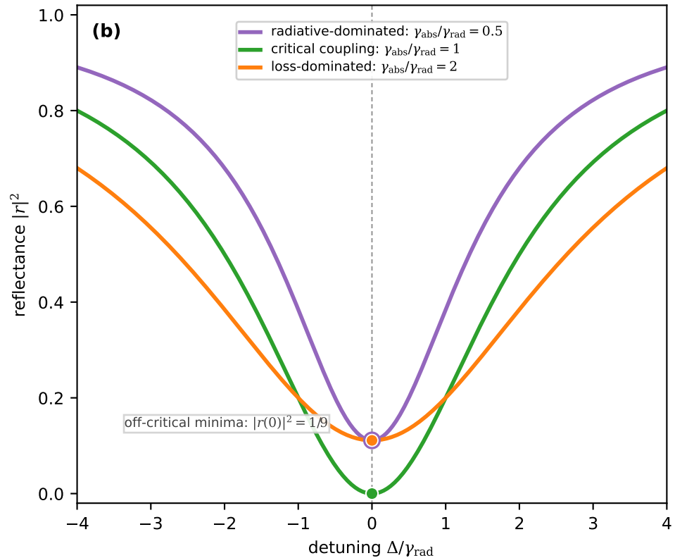
Reflectance spectra: only critical coupling reaches zero
