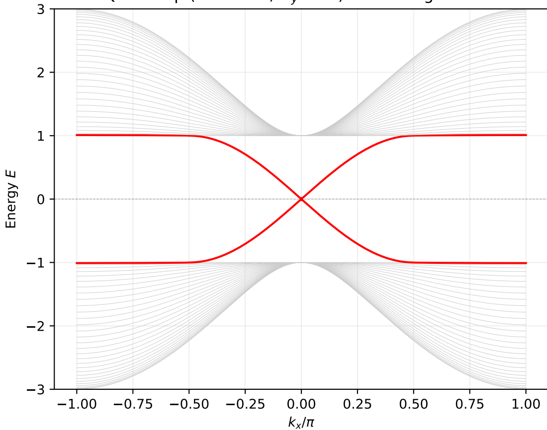
QWZ strip ( m = -1.0 , N_y = 30 ): chiral edge states
