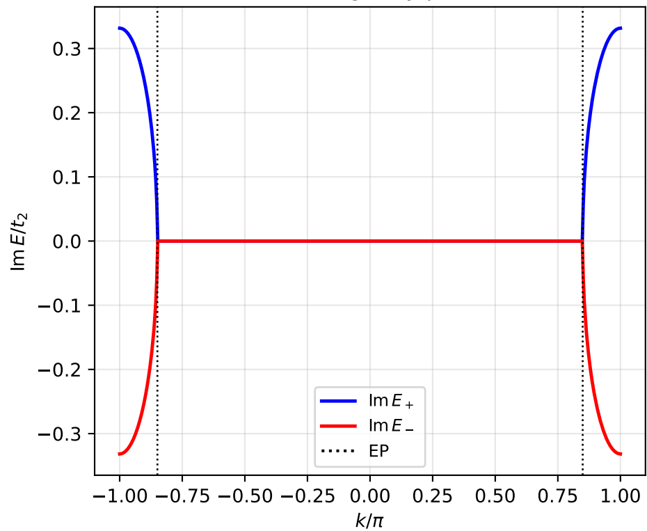
(b) Imaginary part
