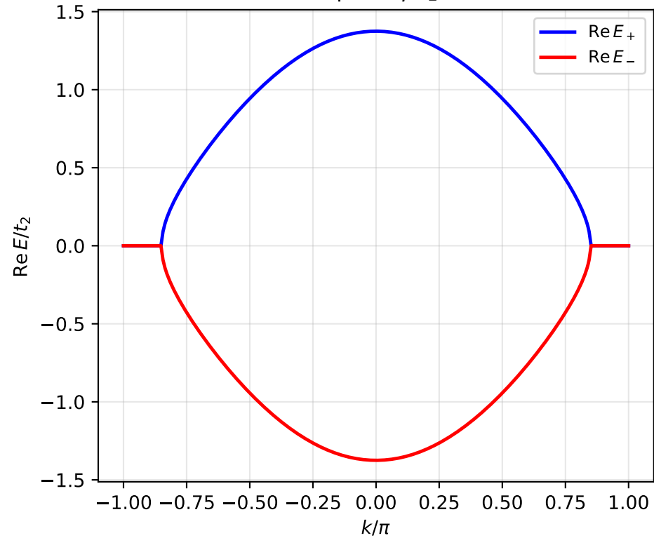
(a) Real part ( \gamma/t_2 = 0.6 )
