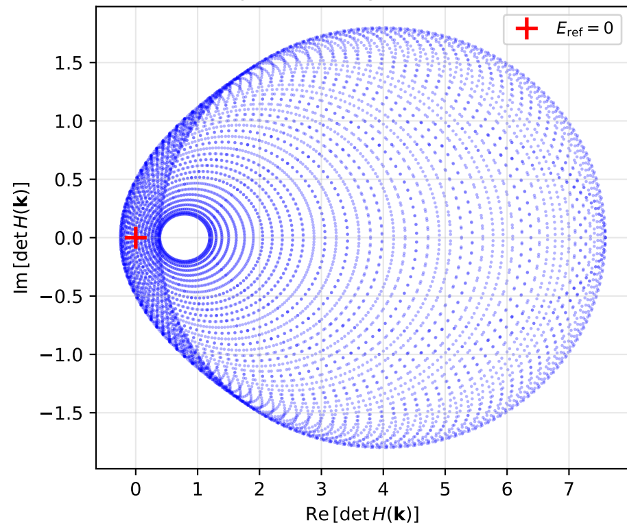
(a) Spectral image of the 2D BZ
