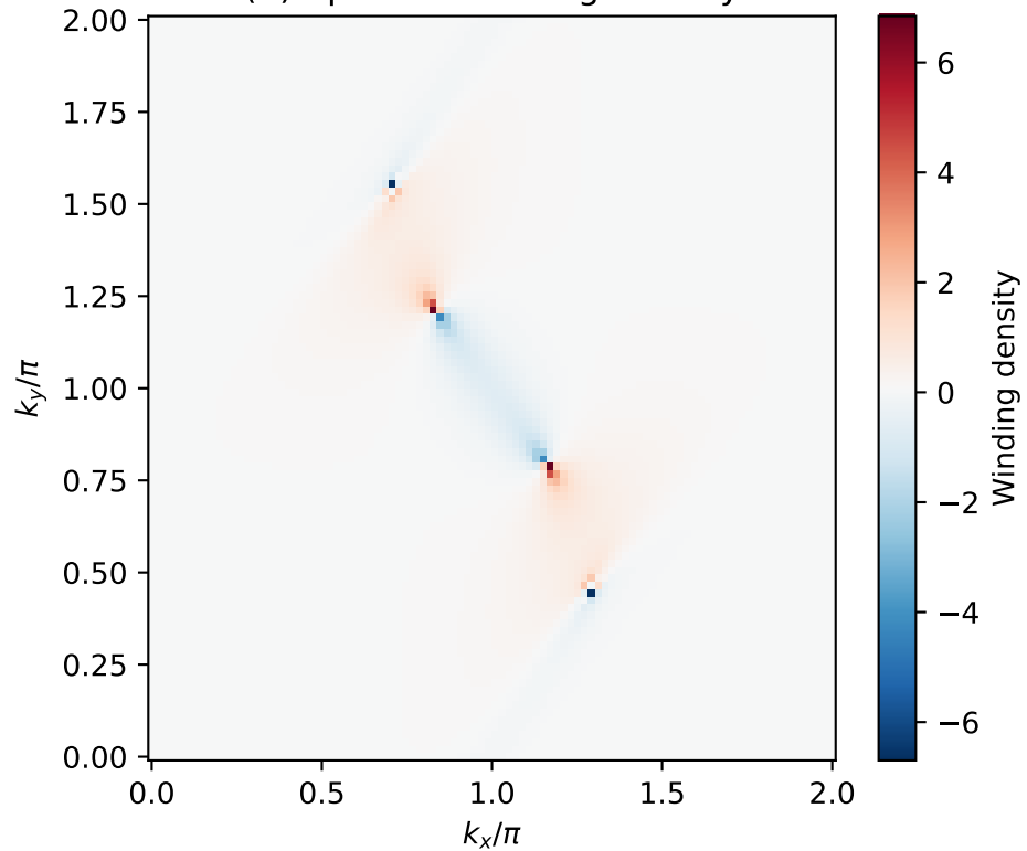
(b) Spectral winding density
