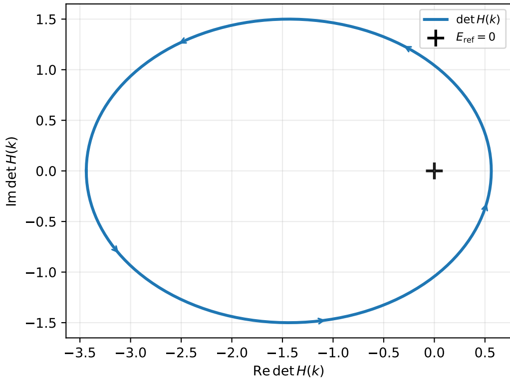
(a) Determinant loop: W = 1.000
