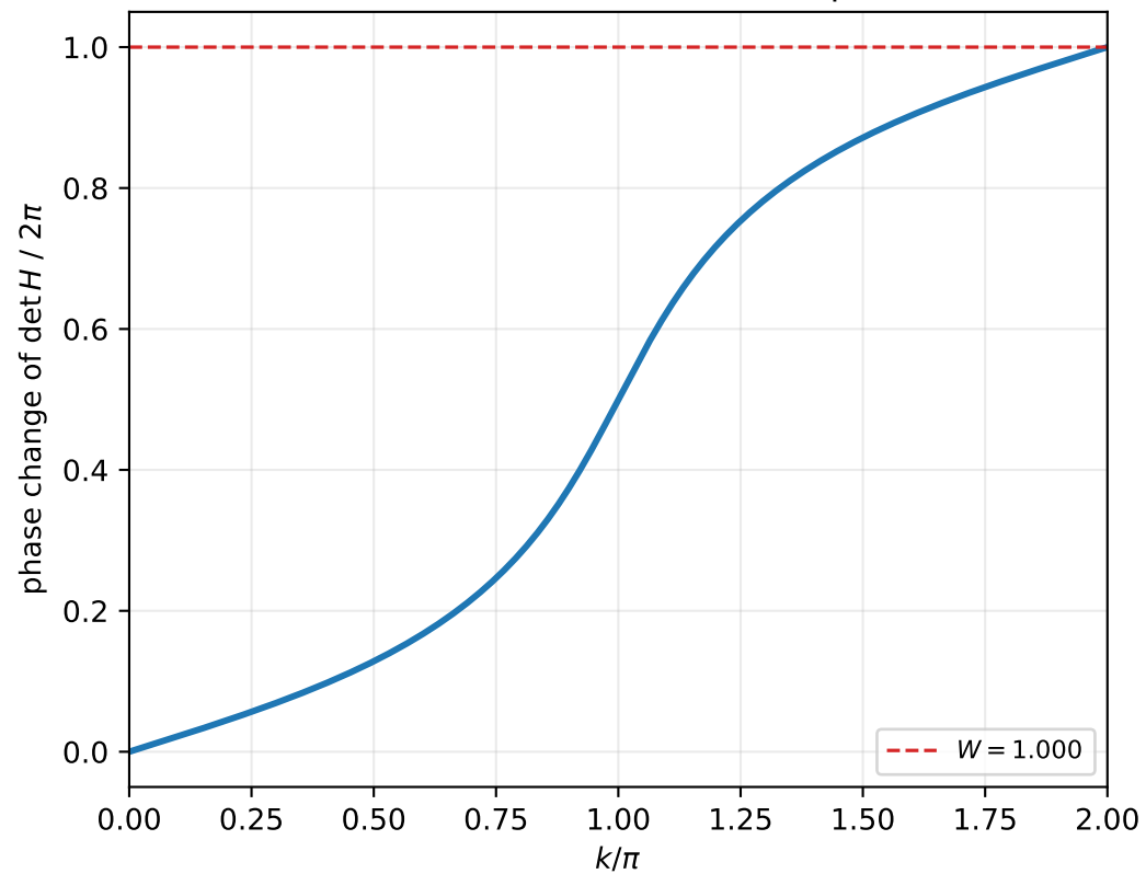
(b) Accumulated determinant phase
