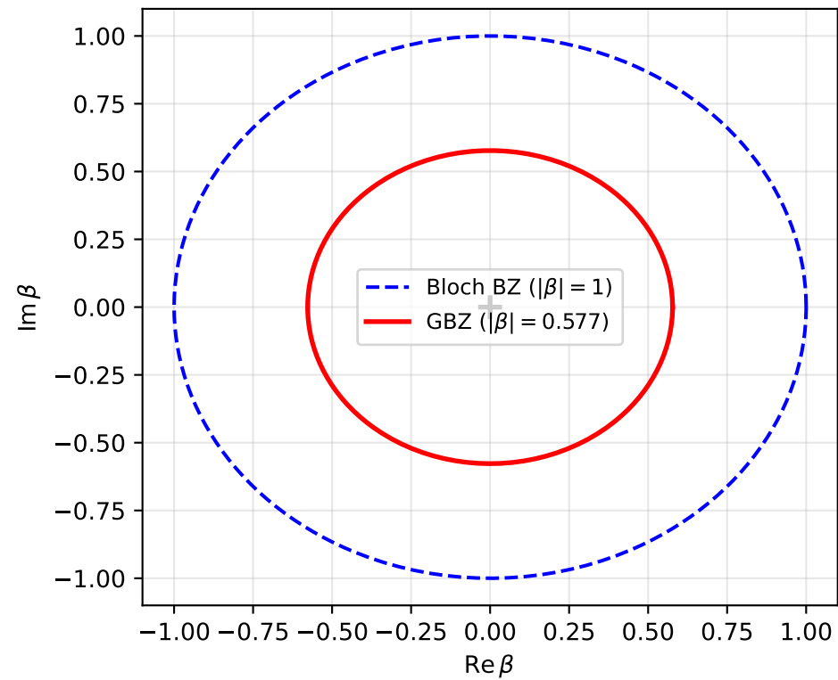
(a) \beta -plane: Bloch vs GBZ
