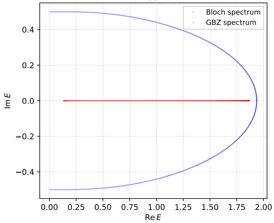
(b) Energy spectra
