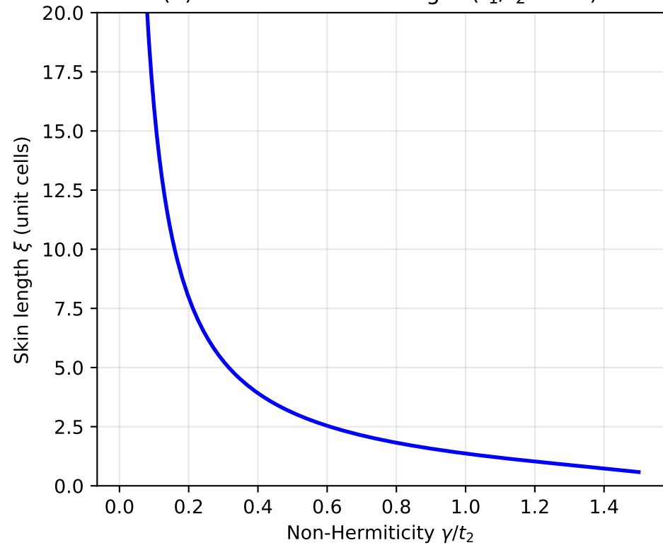
(a) Skin localisation length ( t_1/t_2 = 0.8 )
