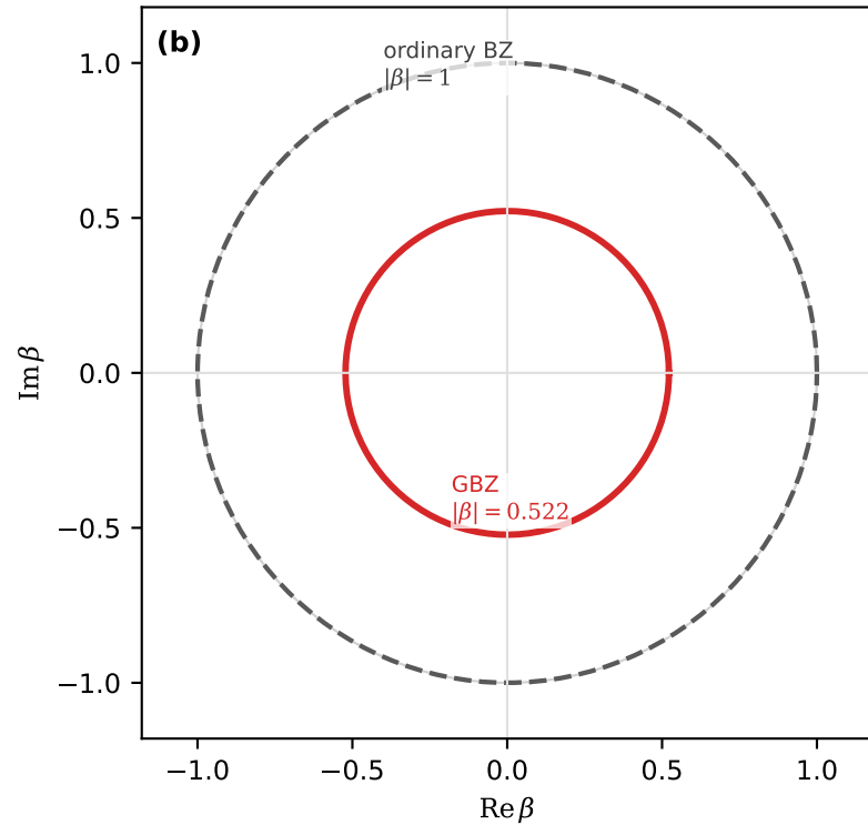
Generalized Brillouin zone
