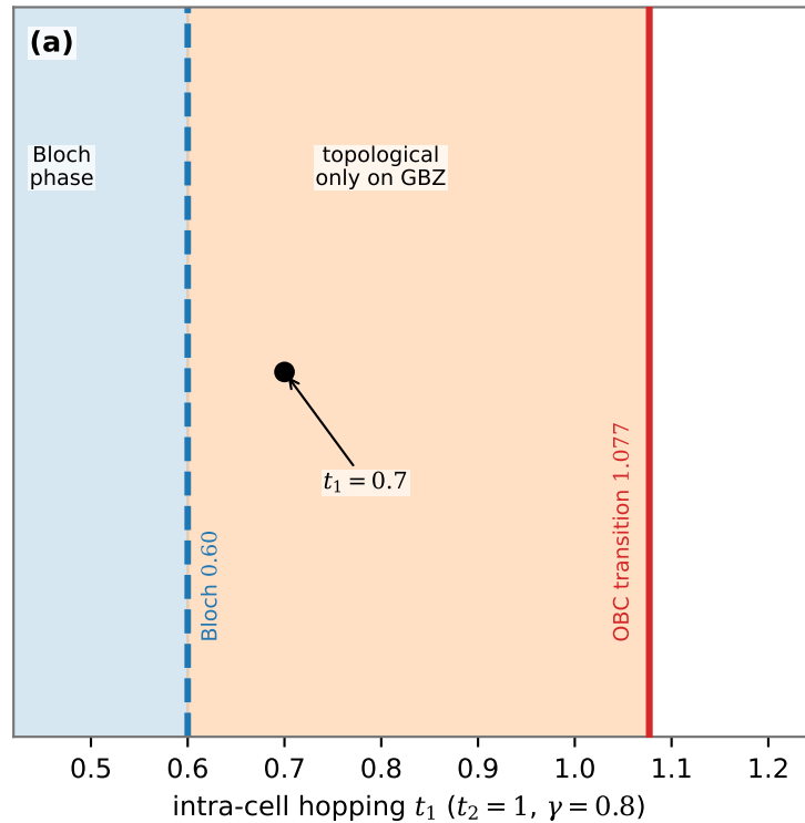
Bloch boundary misses OBC transition
