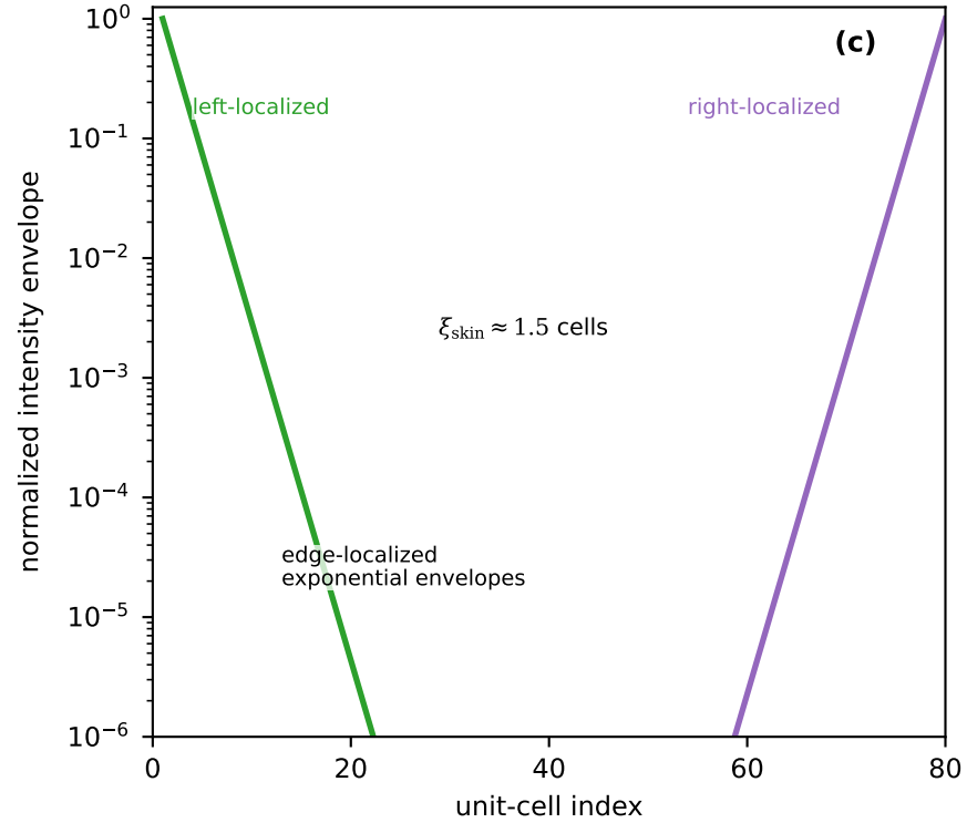
OBC eigenstate intensity envelopes
