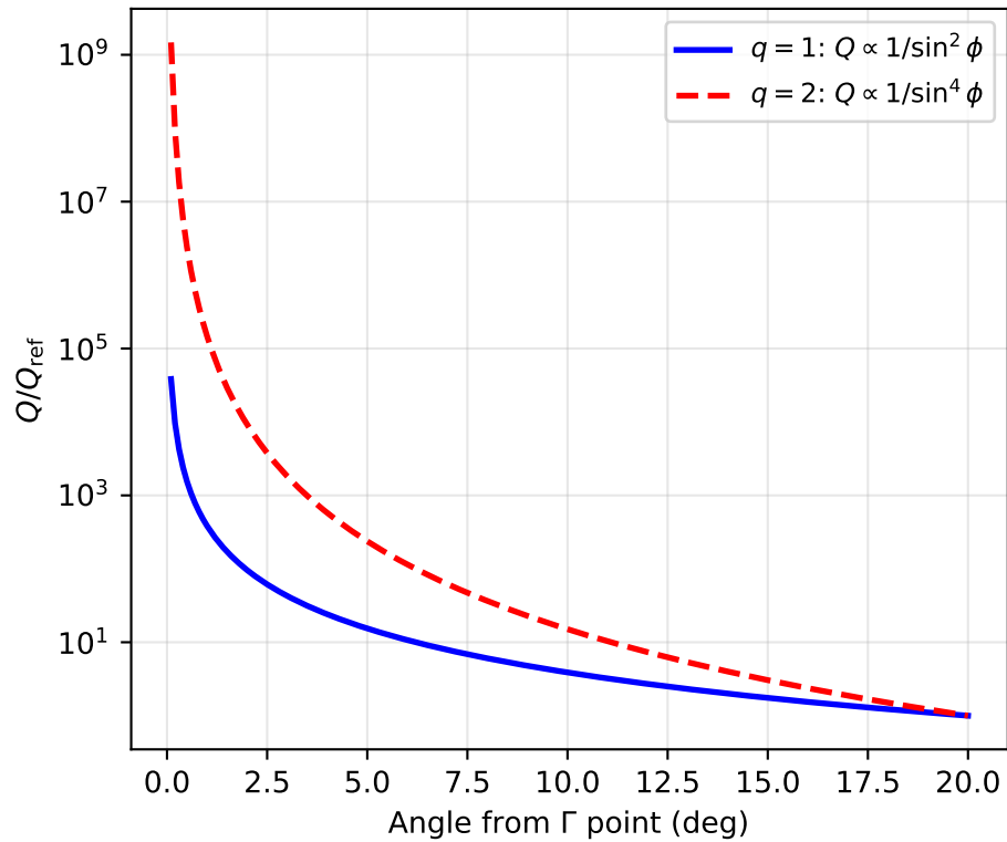
(b) Q -factor divergence near BIC
