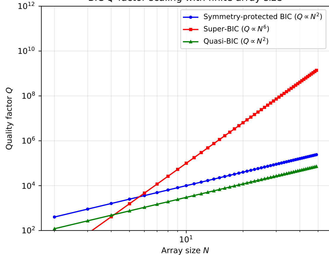
BIC Q-factor scaling with finite array size
