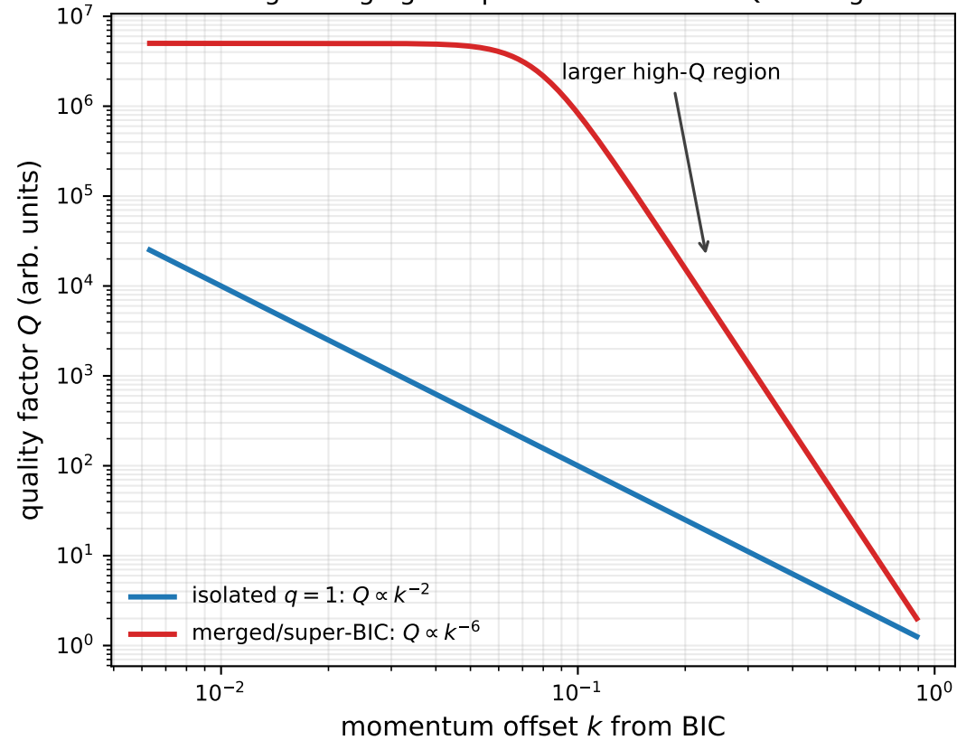
Charge merging steepens the finite-size Q scaling
