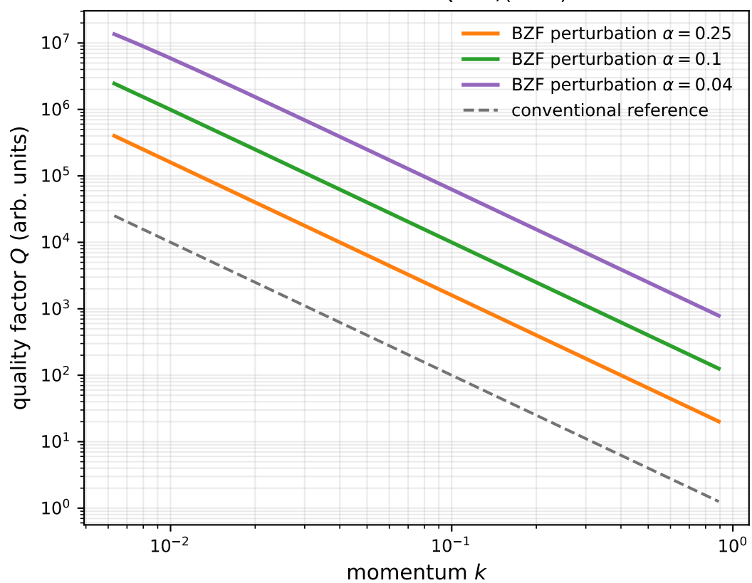
BZF-BIC control: Q \sim 1/(\alpha^2 k^2)
