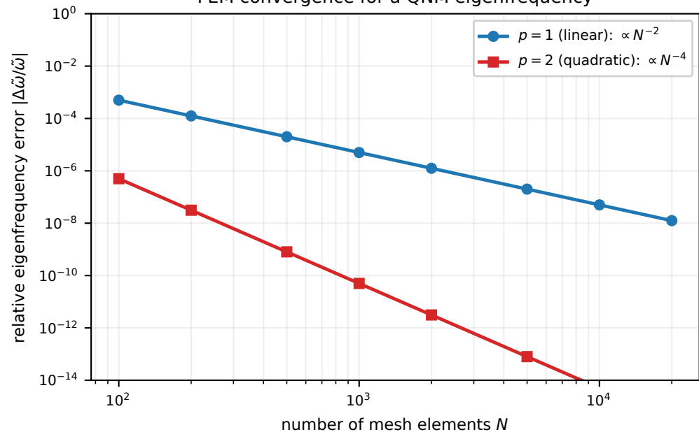
FEM convergence for a QNM eigenfrequency
