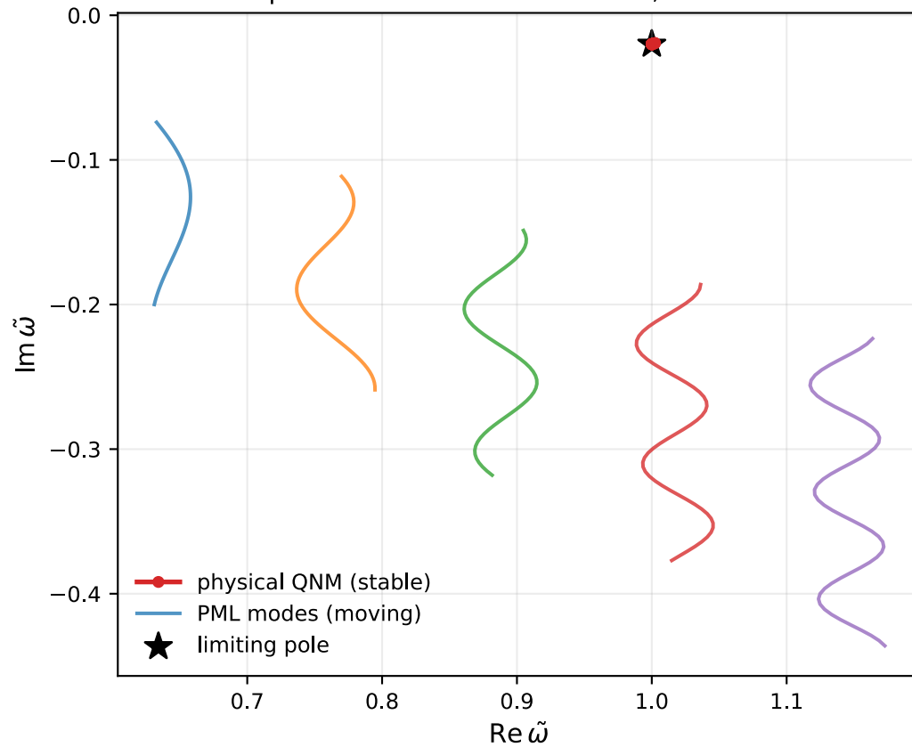
PML sweep: true resonances are stable; PML modes move
