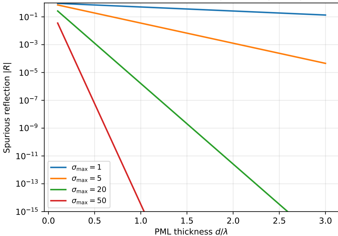
PML reflection vs thickness (quadratic grading)
