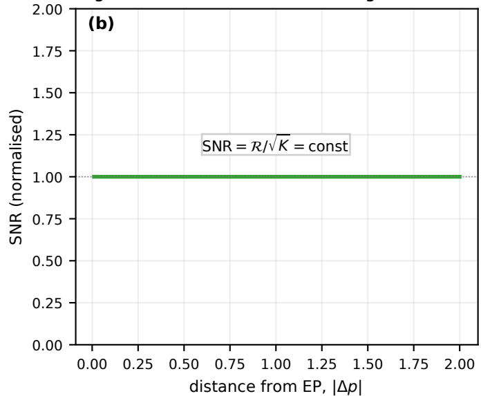
Signal-to-noise ratio: EP advantage cancelled
