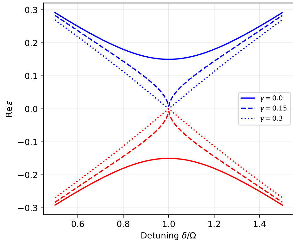
(a) Floquet quasi-energy (real)
