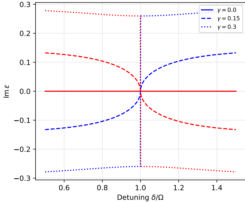
(b) Floquet quasi-energy (imaginary)
