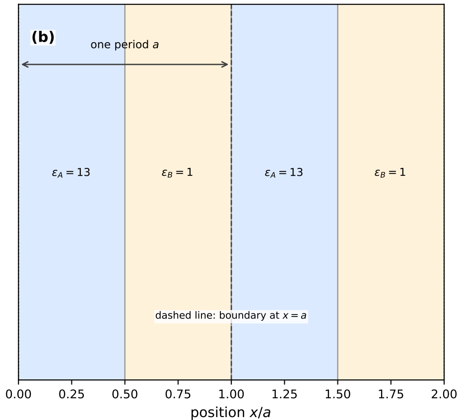
Real-space unit-cell geometry
