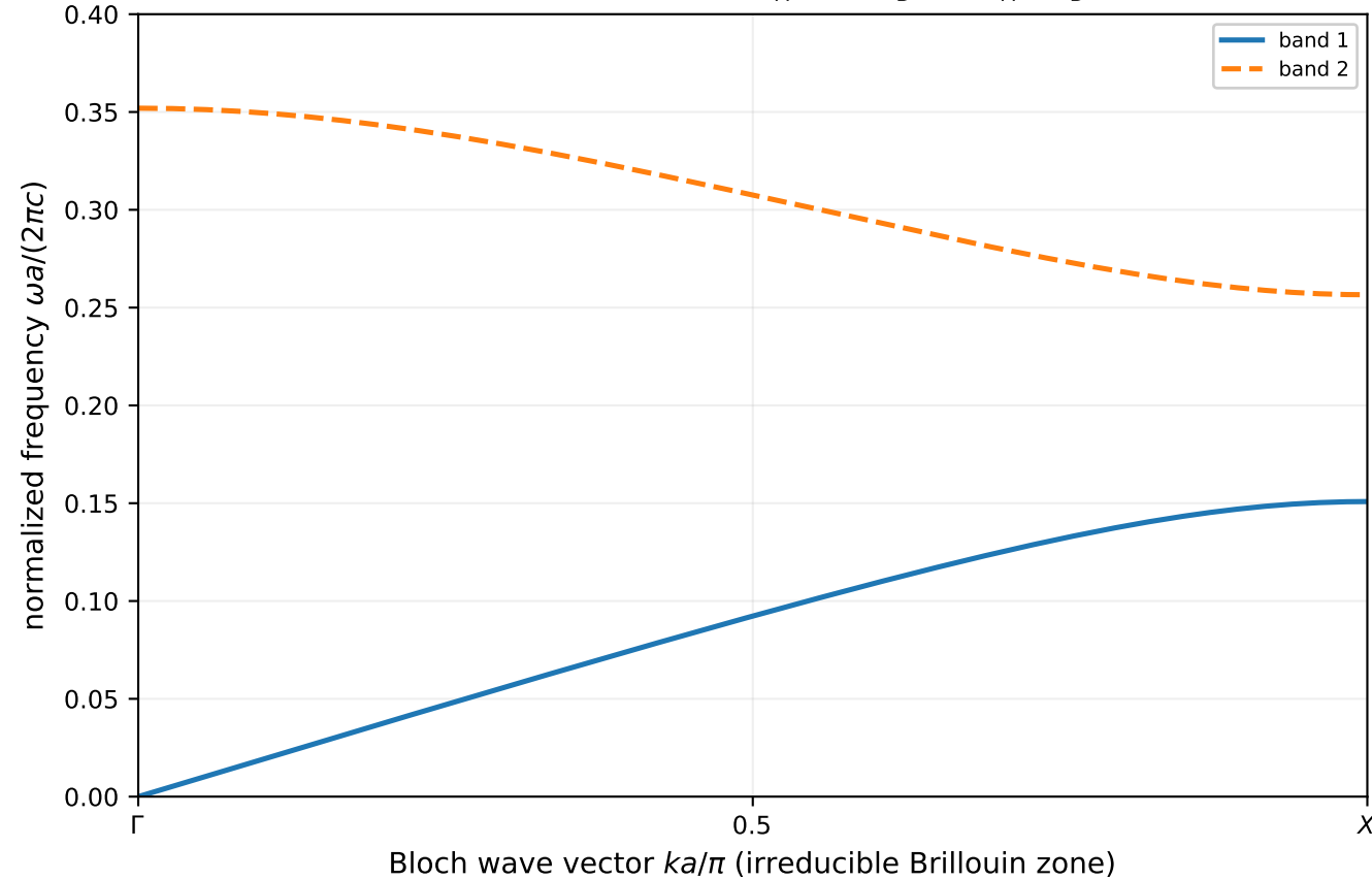
(a) Scalar transfer-matrix bands ( \epsilon_A = 13 , \epsilon_B = 1 , d_A = d_B = a/2 )
