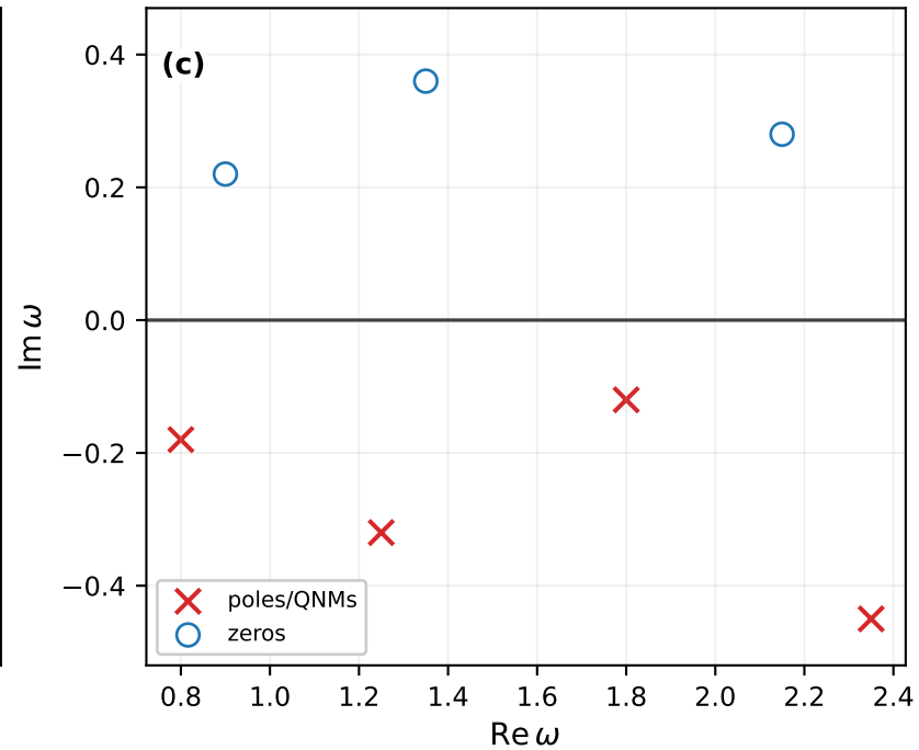
Open/lossy system complex poles and zeros
