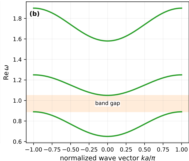
Periodic medium real bands and gaps
