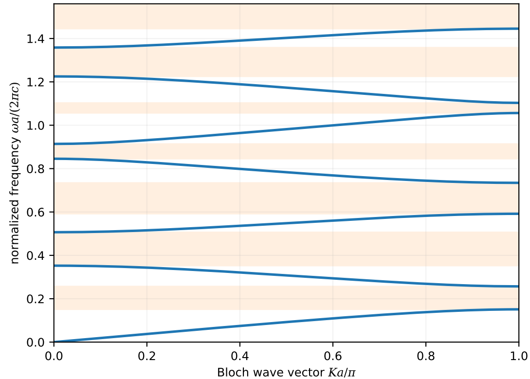
(a) Pass bands and stop bands
