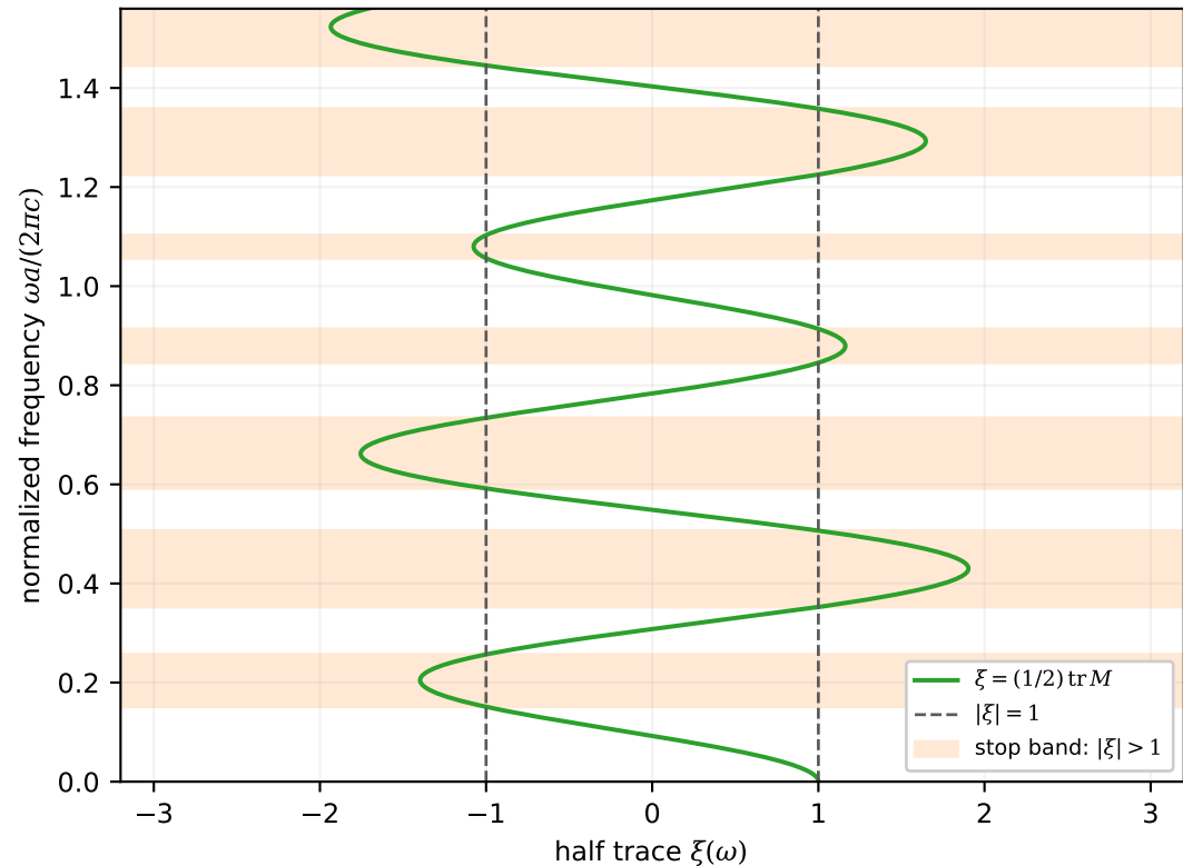
(b) Same gaps from the trace criterion
