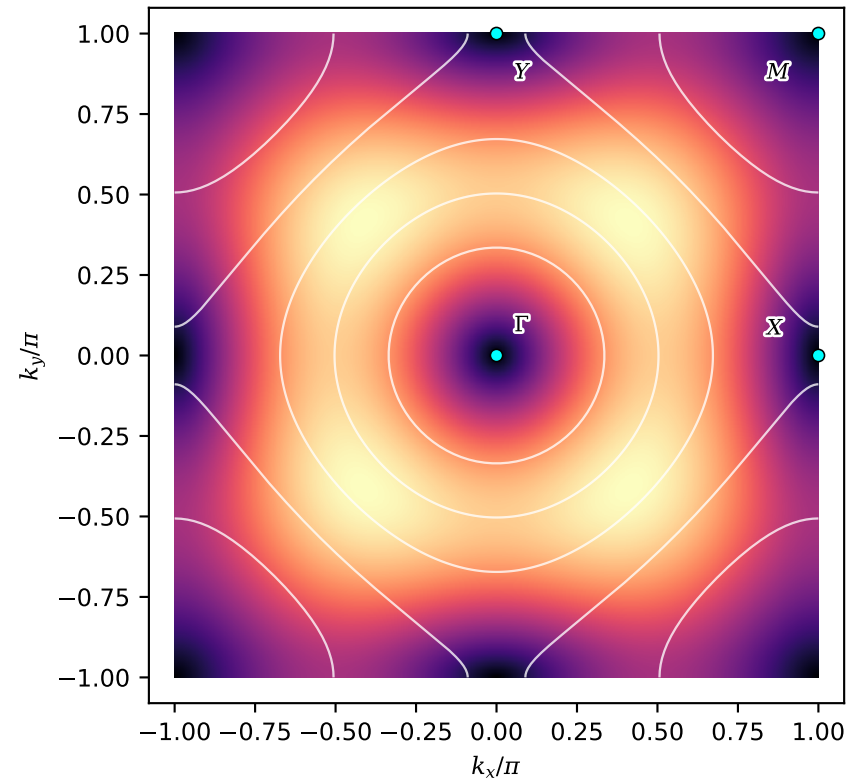
(a) Group speed; white curves are \omega contours
