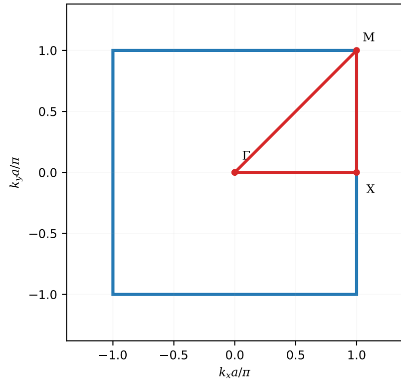
Square-lattice first BZ
