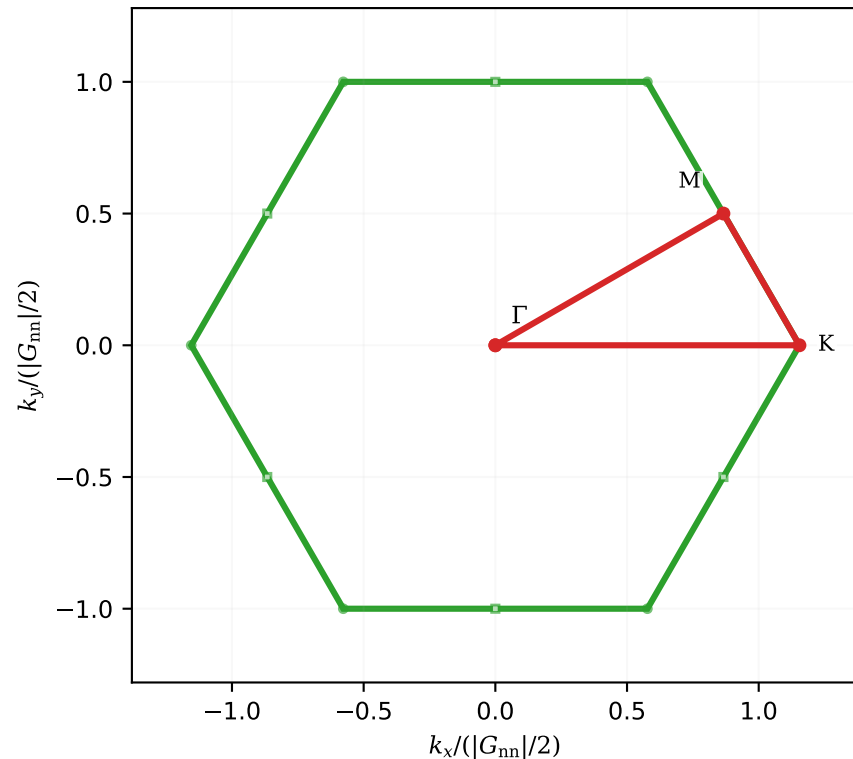
Hexagonal BZ of triangular lattice
