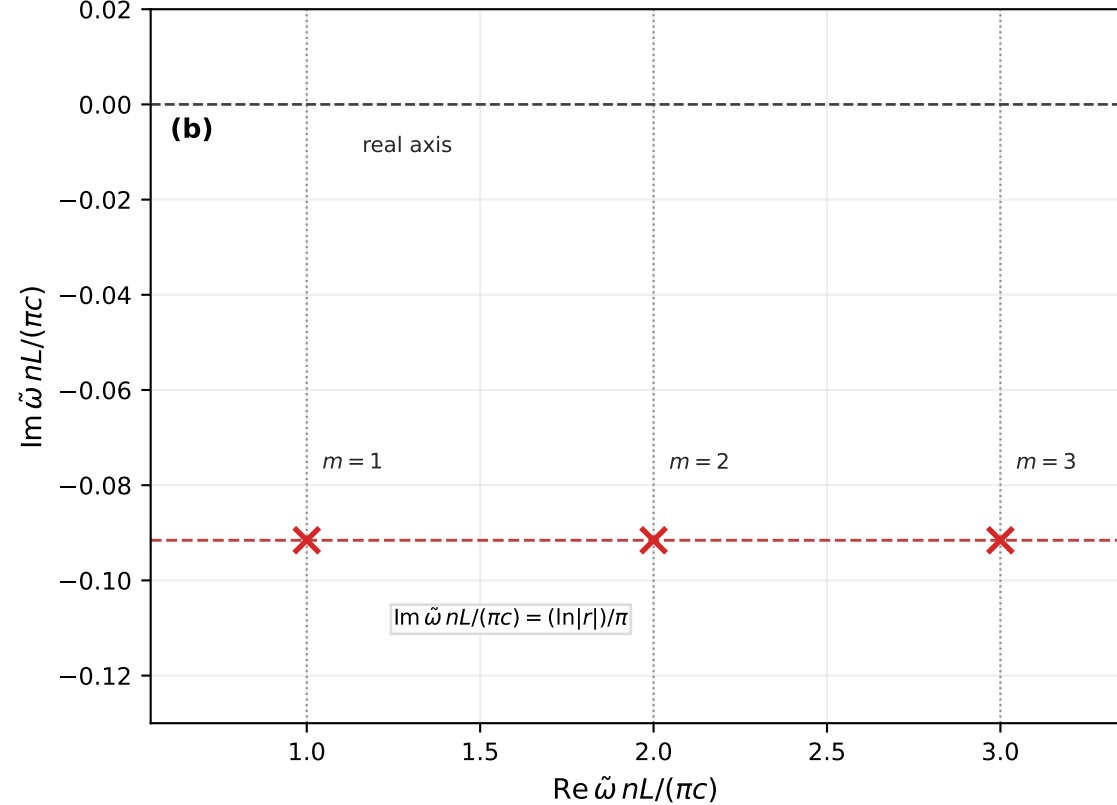
First three S-matrix poles
