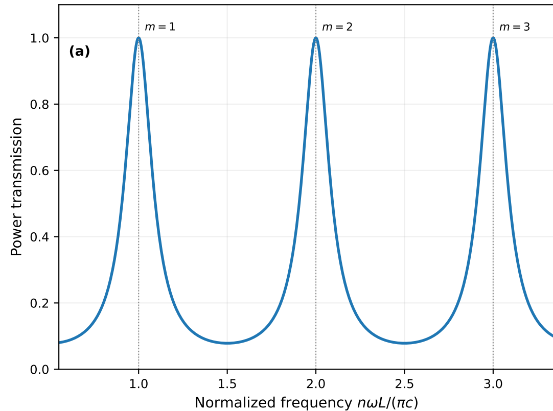
Airy transmission, |r| = 0.75
