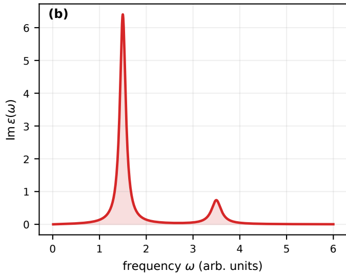
Absorption (Kramers--Kronig partner)
