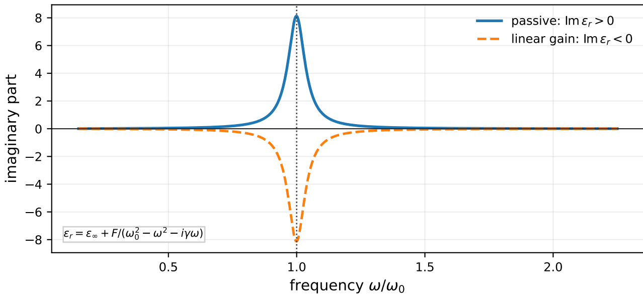
Absorption and gain from the same causal resonance
