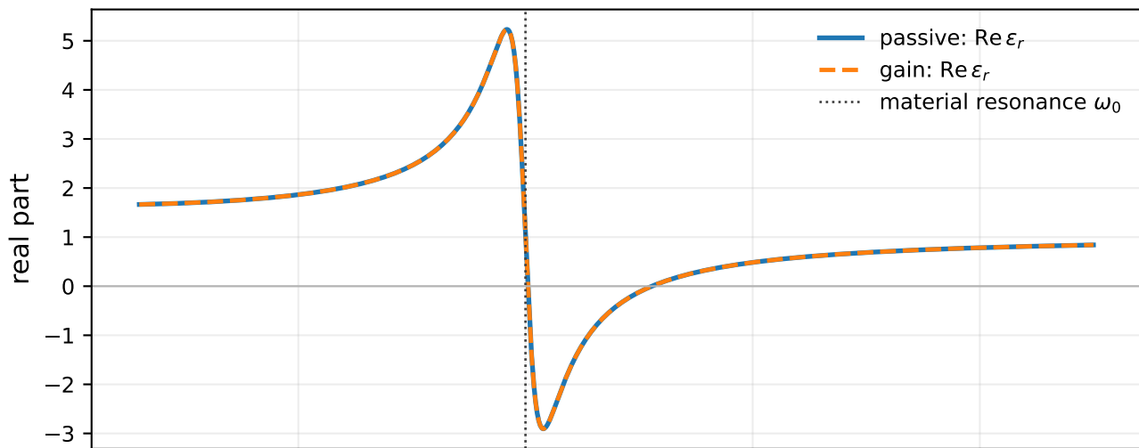
Absorption and gain from the same causal resonance
