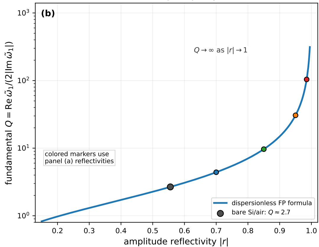
Fundamental-pole quality factor
