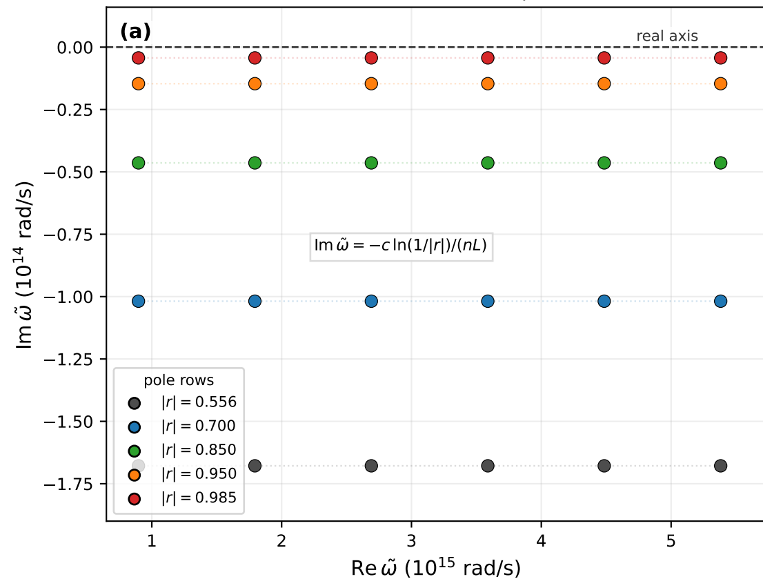
Pole rows from the round-trip condition
