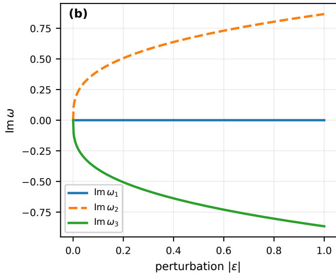
Imaginary parts: three-fold splitting
