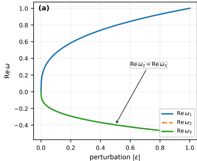
EP 3 eigenvalue splitting: \omega \sim \varepsilon^{1/3}
