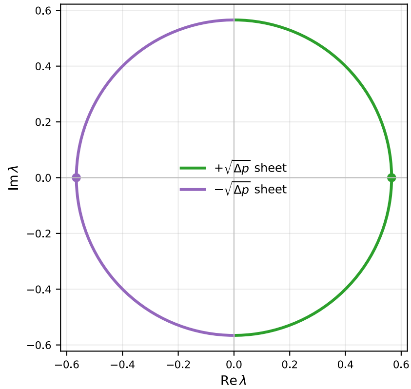
One loop around an EP exchanges the two eigenvalue sheets
