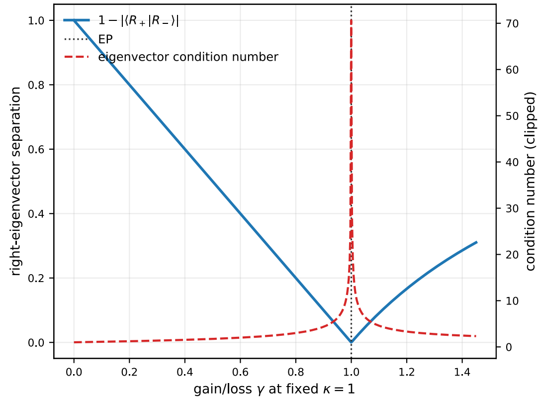
Eigenvectors coalesce and become ill-conditioned at the EP
