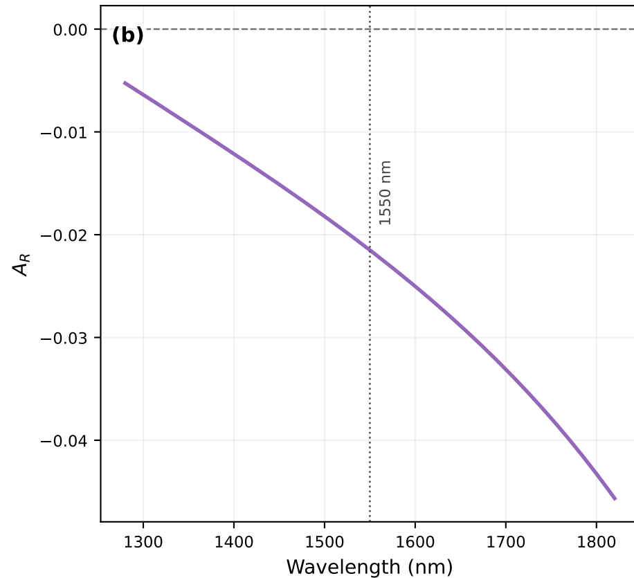
Finite stack from PT-symmetric bilayer unit cells Directional asymmetry A_R(\lambda)
