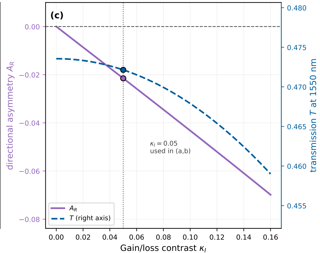
A_R(1550\text{ nm}) and T sweep
