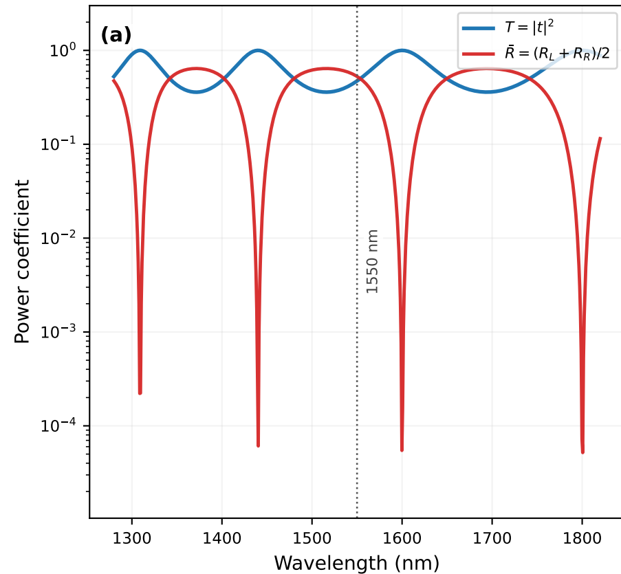
Finite-stack spectra ( N = 6 )
