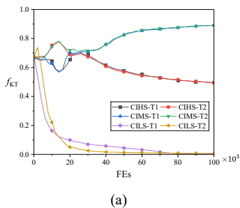
Fig. S3. The KT frequency variation curves for the three groups on high-dimensional scenarios. (a) CI group; (b) PI group; (c) NI group.
