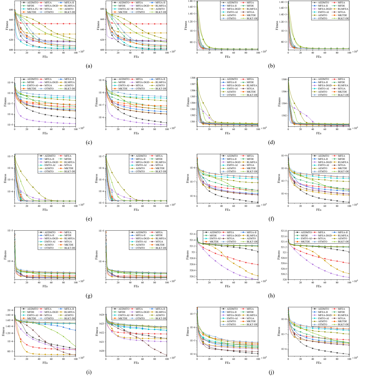
Fig. S2. Convergence curves on all tasks in CEC2022. Subplots (a)-(j) correspond to the ten benchmarks, respectively.
