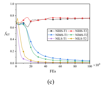
Fig. S3. The KT frequency variation curves for the three groups on high-dimensional scenarios. (a) CI group; (b) PI group; (c) NI group.
