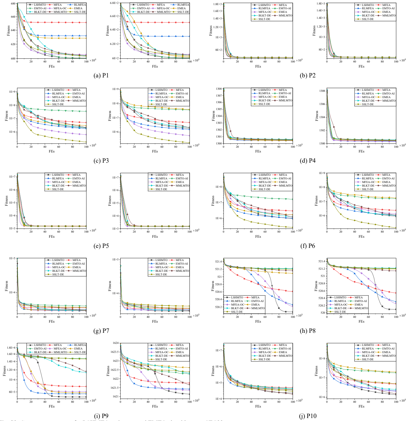
Fig. S2. Convergence curves for LSHMTO and compared EMTO algorithms on CEC22.
