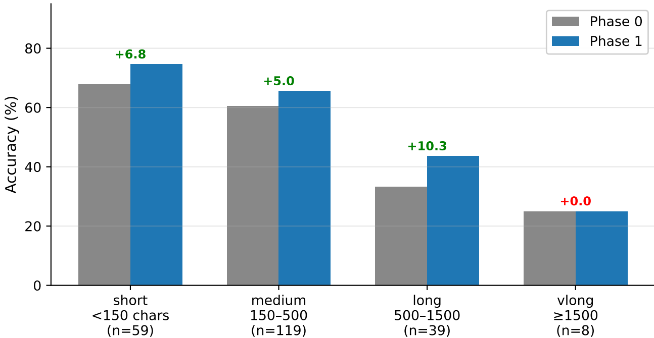
Accuracy degrades on long questions (validation, n=225)
