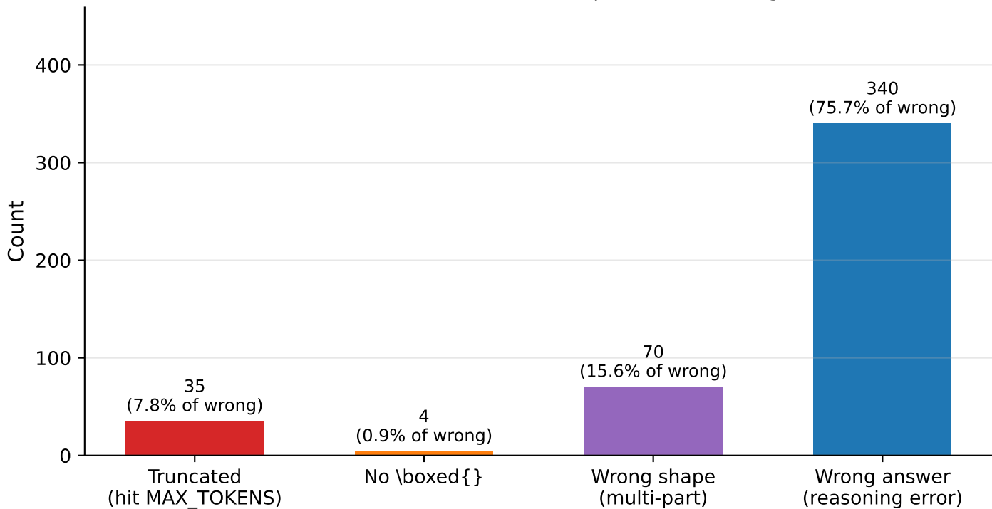
Failure mode breakdown on Phase 1 (full public, 449 wrong / 1126 total)
