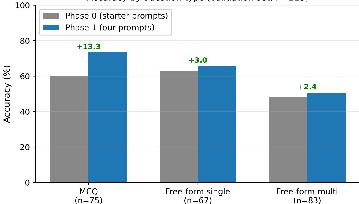
Accuracy by question type (validation set, n=225)
