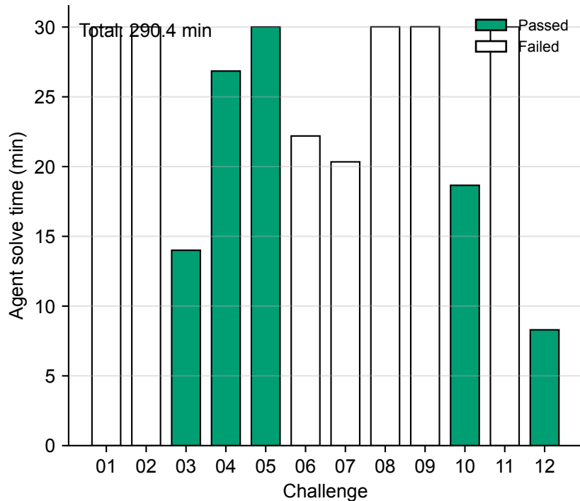
Solver wall time
