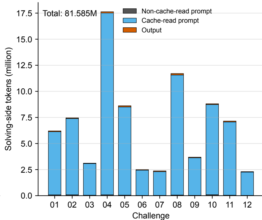
Solver token use
