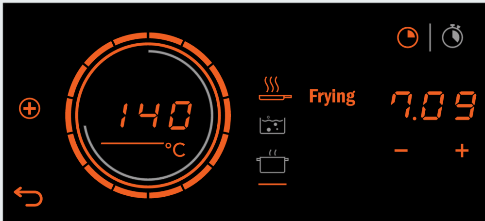
Figure 44: The visualisation of the timer function with numbers.
