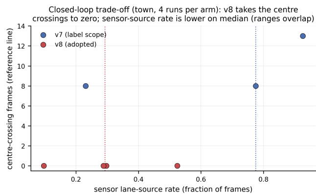
Fig. 14. Closed-loop trade-off: centre crossings versus sensor lane-source rate, four runs per arm.
