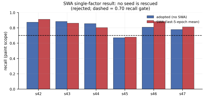
Fig. 12. Rejected single factor: last-five-epoch weight averaging rescues no seed (paint-scope recall).
