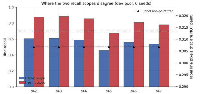
Fig. 7. Per-seed label-scope versus paint-scope recall with the non-paint fraction of label line pixels (development pool).
