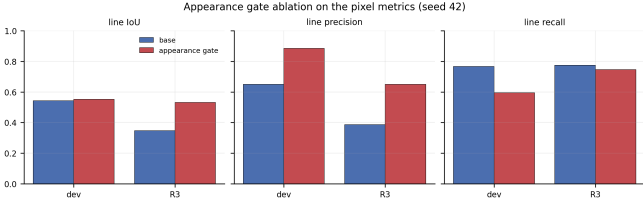
Fig. 9. Appearance-gate ablation on the pixel metrics (line IoU, precision, recall) for both sets, seed 42.
