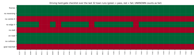
Fig. 15. Driving hard-target checklist over the most recent town runs (green = pass, red = fail; an unmeasured target counts as fail).
