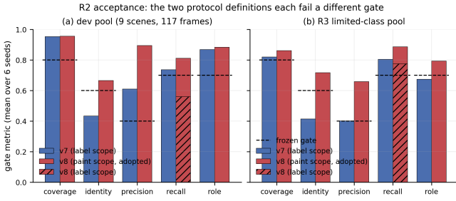
Fig. 6. Gate metrics against frozen thresholds for the two protocol definitions, development pool (a) and limited-class pool (b).
