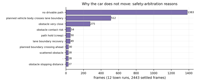
Fig. 24. Why the car does not move: safety-arbitration reasons over 2443 settled frames.
