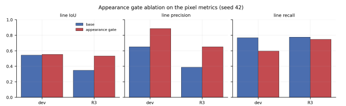
Fig. 15. Appearance-gate ablation on the pixel metrics (line IoU, precision, recall) for both sets, seed 42.
