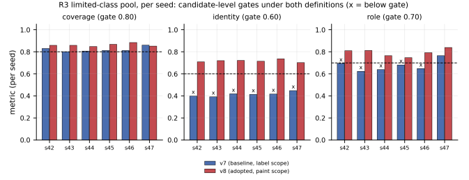
Fig. 10. R3 limited-class pool, per seed: the three candidate-level gates under both definitions, drawn from the same verdict files as Table I (x = below gate).
