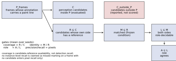
Fig. 3. Counting contract (schematic): every ratio has an explicit numerator and denominator, over the frozen counter definitions; coverage is candidate-reference availability, not detection recall.
