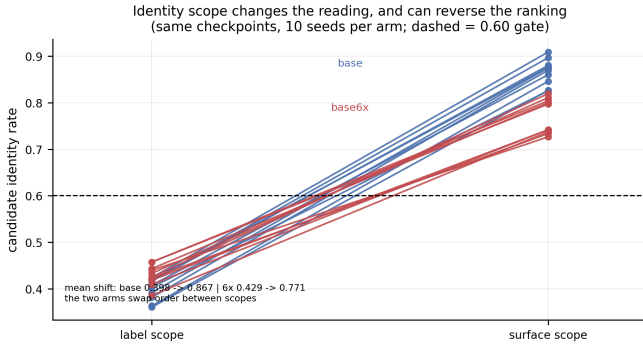
Fig. 12. Identity scope changes the reading and can reverse the ranking: 20 checkpoints (two arms, ten seeds each) read in label and surface scope.
