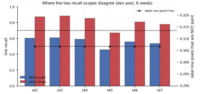
Fig. 13. Per-seed label-scope versus paint-scope recall with the non-paint fraction of label line pixels (development pool).
