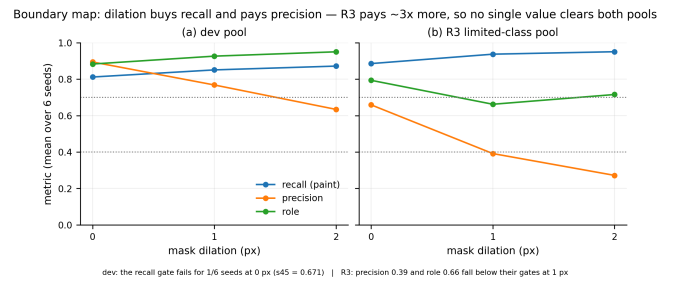
Fig. 14. Boundary map: dilation buys recall and pays precision; the limited-class set pays about three times more.
