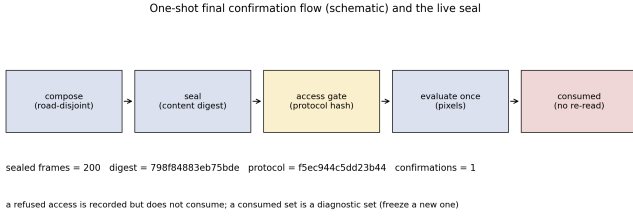
Fig. 6. One-shot final-confirmation flow (schematic) with the live seal.
