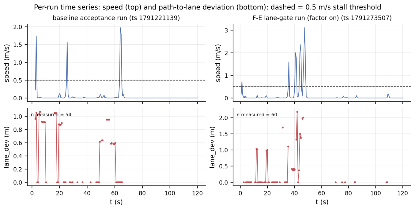
Fig. S24. Per-run time series (speed top, path-to-lane deviation bottom) for a baseline acceptance run and an F-E lane-gate run.
