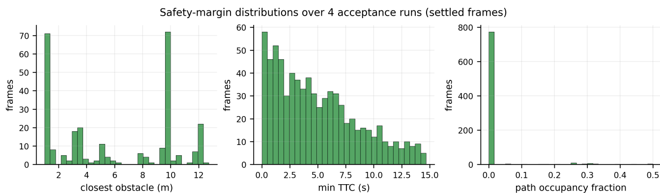
Fig. S27. Safety-margin distributions (closest obstacle, minimum time-to-collision, path occupancy) over four acceptance runs.
