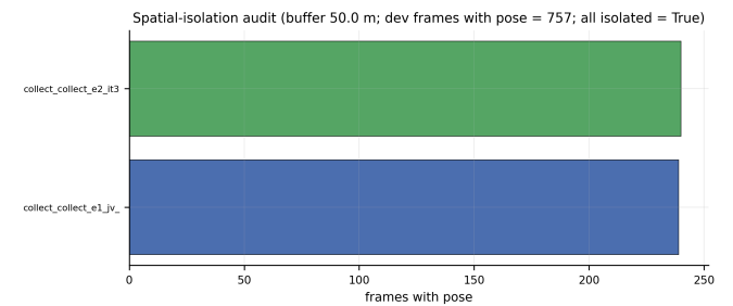
Fig. S16. Spatial-isolation audit: every candidate collection against the development anchors under a 50 m buffer.
