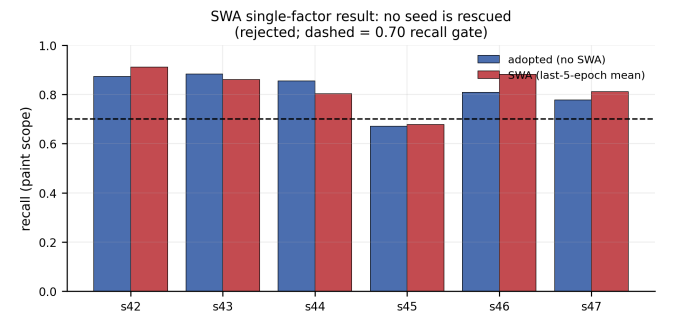
Fig. S10. SWA single-factor result: no seed is rescued by last-five-epoch averaging.
