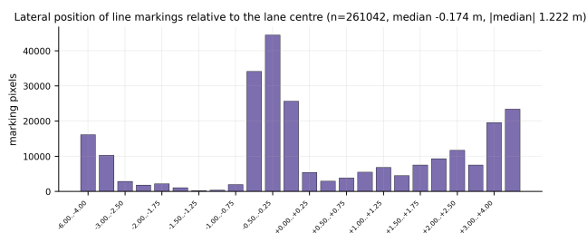
Fig. S42. Panel (d) of the main-text rigour and audits composite. Lateral position of line markings relative to the lane centre, pooled over the human-revised development pool.
