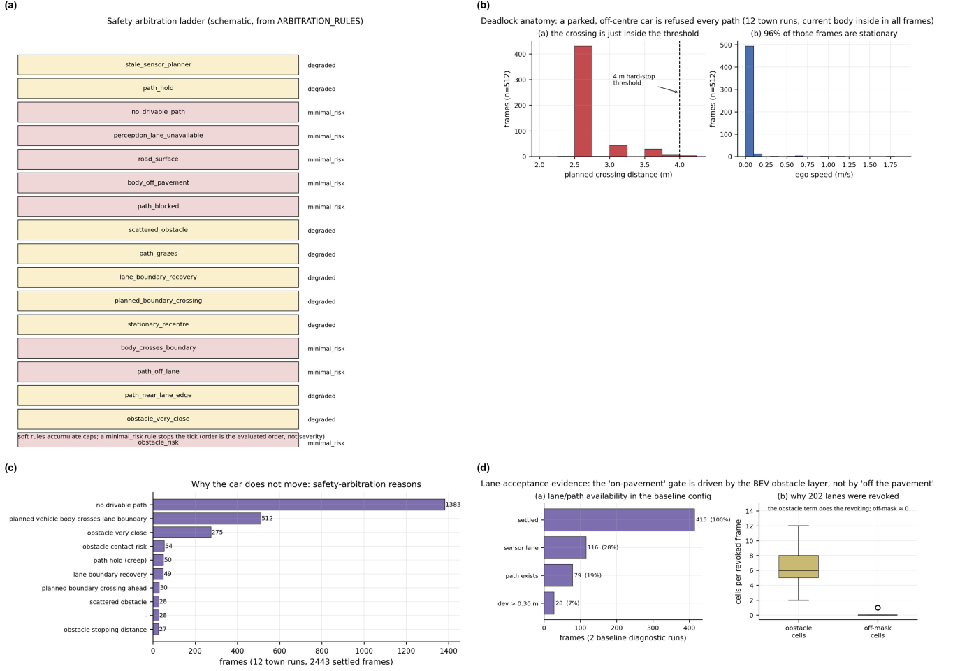
Fig. 2. Why the car does not move: (a) the safety arbitration ladder (schematic), (b) the deadlock anatomy, (c) the arbitration reasons over 2443 settled frames, (d) the lane-acceptance evidence — the on-pavement gate is driven by the BEV obstacle layer.
