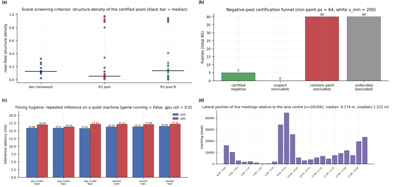
Fig. 3. Rigour and audits: (a) the scene-screening criterion (near-field structure density), (b) the negative-pool certification funnel, (c) the timing-hygiene retest, (d) the measured lateral geometry of the reference markings.
