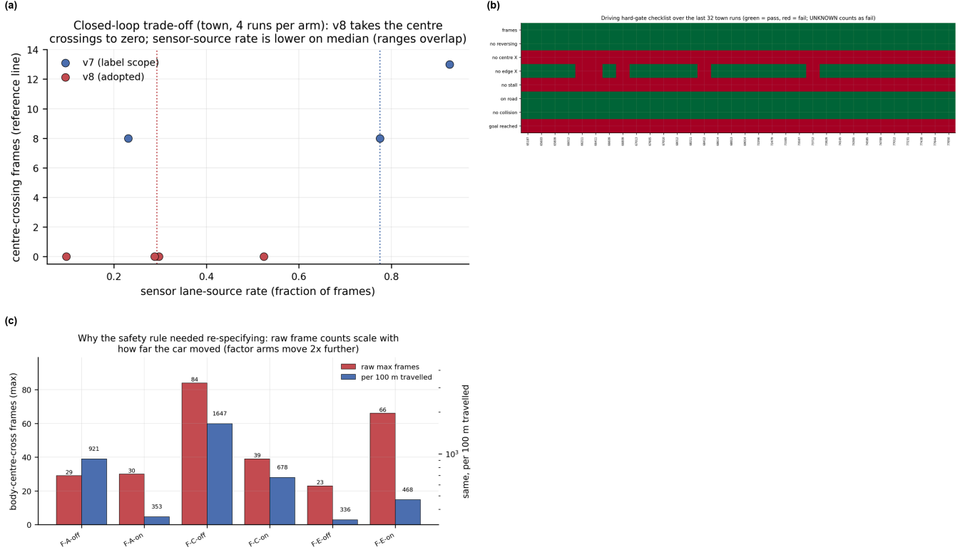
Fig. 7. Closed loop: (a) centre crossings versus sensor lane-source rate for the two definitions, (b) the hard-target checklist over the recent town runs, (c) why the safety rule needed re-specifying (raw counts scale with how far the car travelled).
