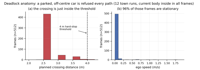
Fig. S36. Panel (b) of the main-text deadlock mechanism composite. Deadlock anatomy: the planned crossing sits just inside the 4 m threshold (a) and the car is stationary in 96% of those frames (b).
