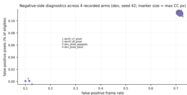
Fig. S20. Negative-side diagnostics across all recorded pixel arms (false-positive frame rate versus false-positive pixel fraction; marker size = largest connected component).
