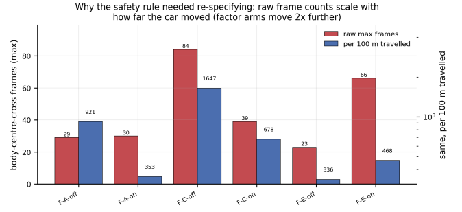
Fig. S34. Panel (c) of the main-text closed loop composite. Raw crossing counts versus the same quantity normalised per 100 m travelled (log scale).
