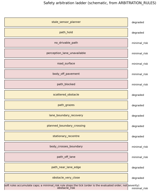
Fig. S35. Panel (a) of the main-text deadlock mechanism composite. Safety arbitration ladder (schematic, from the monitor's rule registry).
