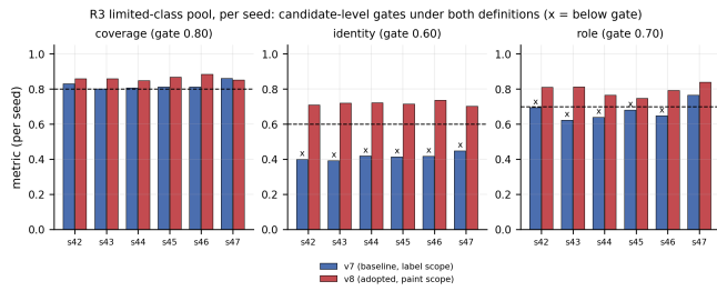
Fig. S22. Panel (b) of the main-text definition sensitivity composite. R3 limited-class pool, per seed: the three candidate-level gates under both definitions, drawn from the same verdict files as Table I (x = below gate).
