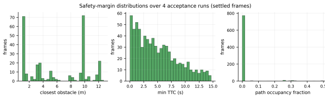
Fig. S27. Safety-margin distributions (closest obstacle, minimum time-to-collision, path occupancy) over four acceptance runs.
