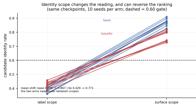
Fig. S24. Panel (d) of the main-text definition sensitivity composite. Identity scope changes the reading and can reverse the ranking: 20 checkpoints (two arms, ten seeds each) read in label and surface scope.
