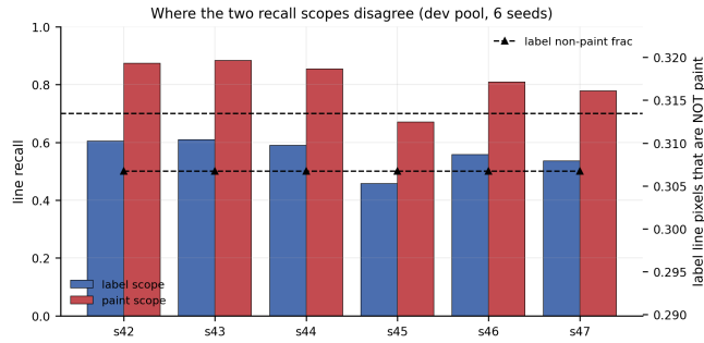
Fig. S23. Panel (c) of the main-text definition sensitivity composite. Per-seed label-scope versus paint-scope recall with the non-paint fraction of label line pixels (development pool).
