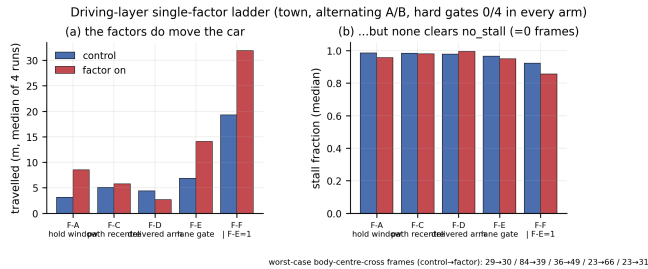
Fig. S1. Driving single-factor ladder: travelled distance (a) and stall fraction (b) per arm, with worst-case body-centre-cross frames.
