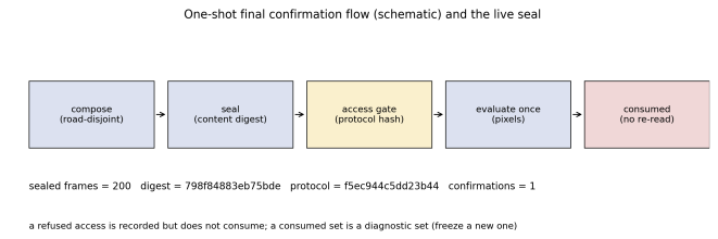
Fig. S20. Panel (d) of the main-text design and contract composite. One-shot final-confirmation flow (schematic) with the live seal.
