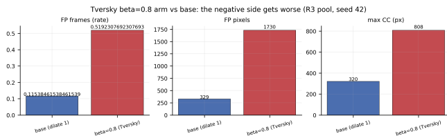
Fig. S17. Tversky \beta=0.8 arm versus base on the negative side (false-positive frames, false-positive pixels, largest connected component).
