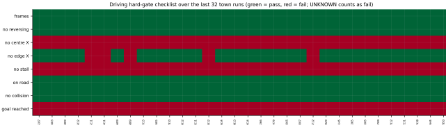
Fig. S33. Panel (b) of the main-text closed loop composite. Driving hard-target checklist over the most recent town runs (green = pass, red = fail; an unmeasured target counts as fail).
