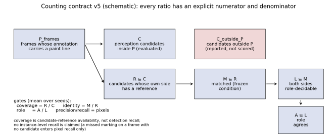
Fig. S18. Panel (b) of the main-text design and contract composite. Counting contract (schematic): every ratio has an explicit numerator and denominator, over the frozen counter definitions; coverage is candidate-reference availability, not detection recall.
