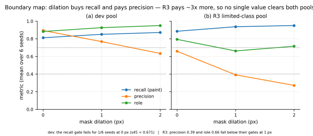
Fig. S25. Panel (a) of the main-text post-processing and composition composite. Boundary map: dilation buys recall and pays precision; the limited-class set pays about three times more.
