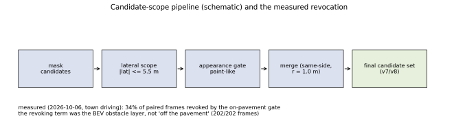
Fig. S17. Panel (a) of the main-text design and contract composite. Candidate-scope pipeline (schematic) with the measured revocation rate.
