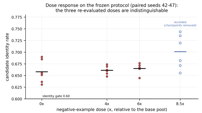
Fig. S28. Panel (d) of the main-text post-processing and composition composite. Dose response of the candidate identity rate (per seed and mean).
