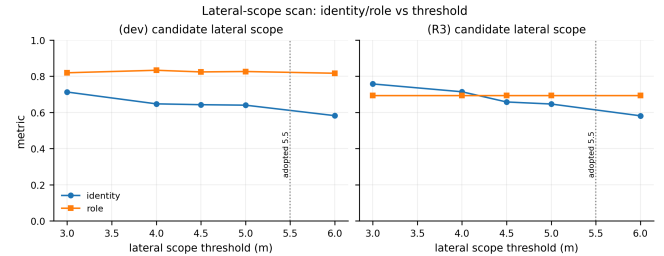
Fig. S27. Panel (c) of the main-text post-processing and composition composite. Lateral-scope scan on both sets: identity and role versus threshold, with the number of retained candidates.
