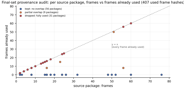
Fig. S31. Panel (c) of the main-text one-shot confirmation composite. Final-set provenance audit: content-level overlap of each source package with the used frame set.
