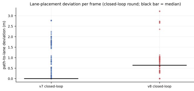
Fig. S26. Per-frame lane-placement deviation in the closed-loop round (v7 vs v8; black bar = median).
