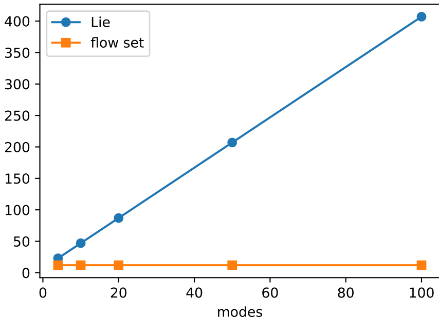
two-qubit depth
