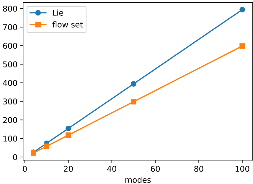
CX count
