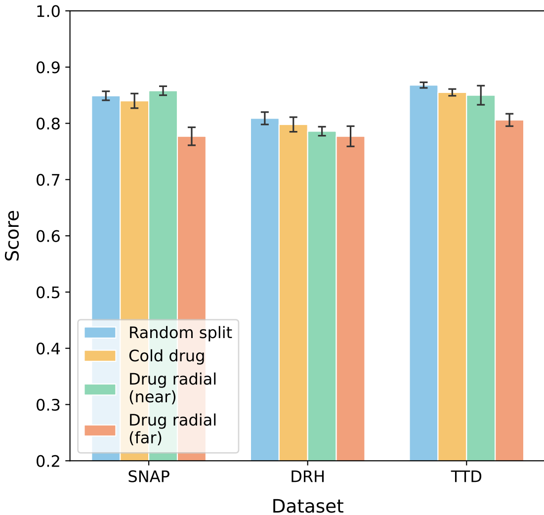
Drug-related: Precision
