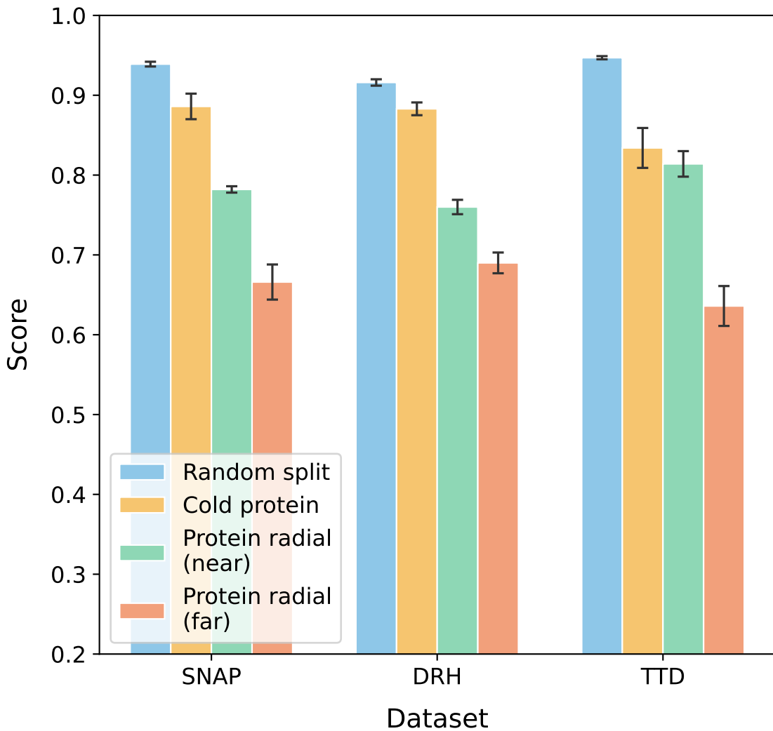
Protein-related: AUROC
