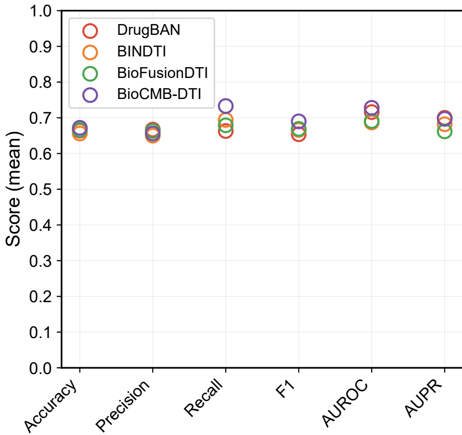
Random split
