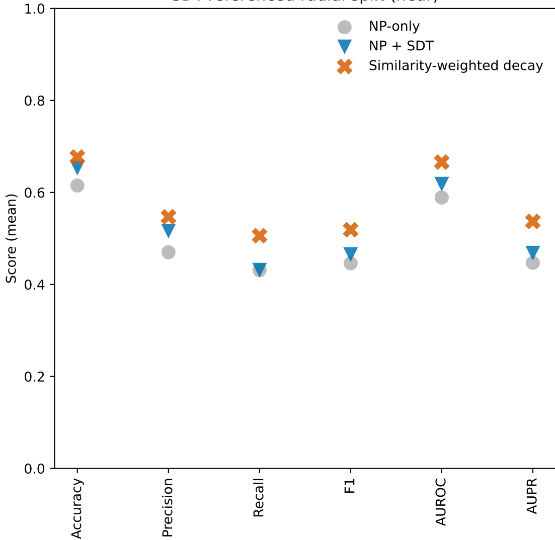
SDT-referenced radial split (near)
