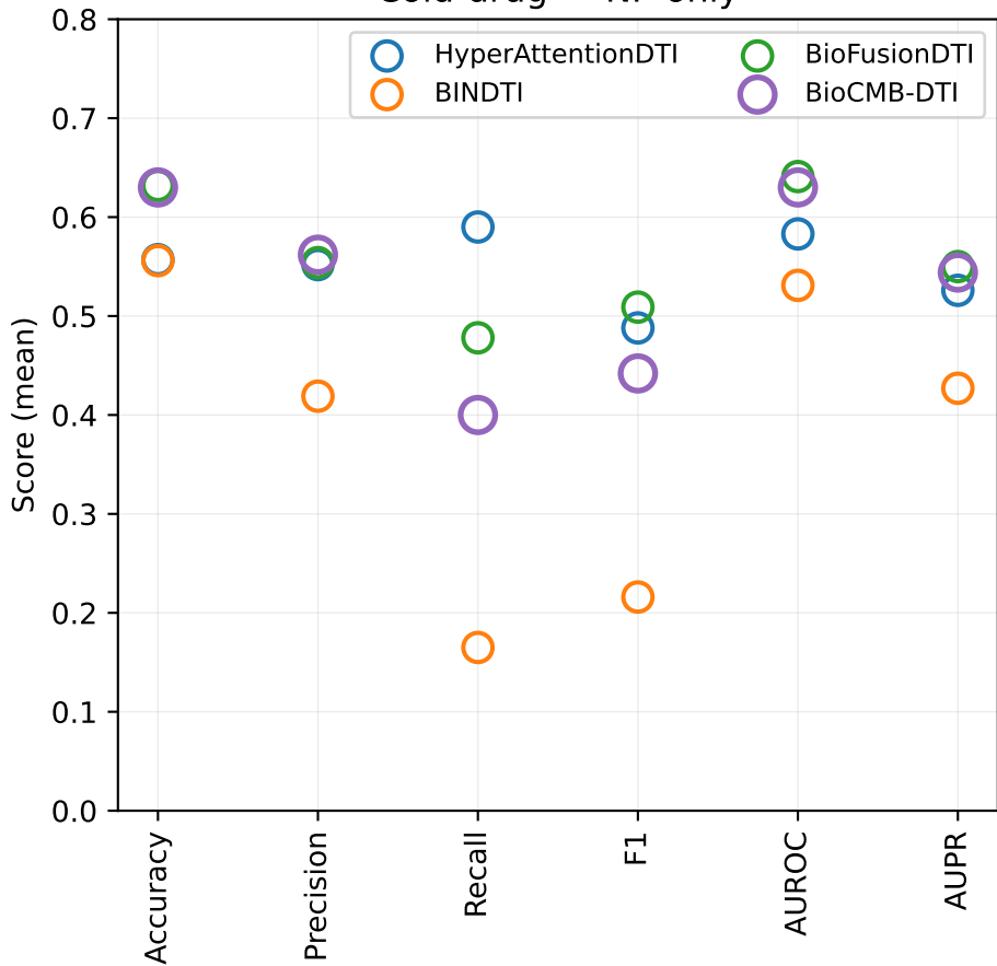
Cold-drug — NP-only
