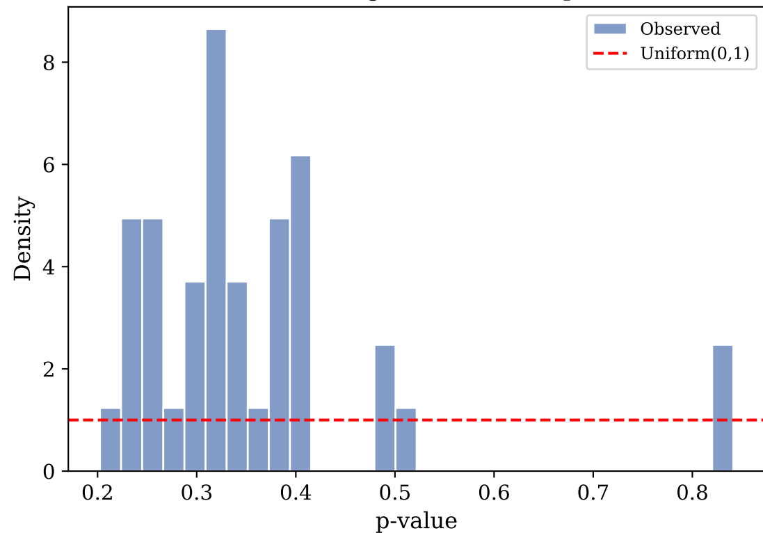
(a) P-value Histogram (Safe Samples, \mathcal{H}_0 )
