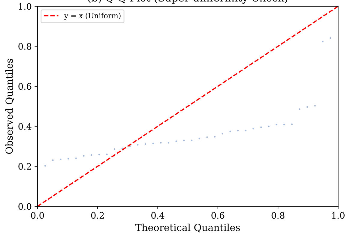
(b) Q-Q Plot (Super-uniformity Check)
