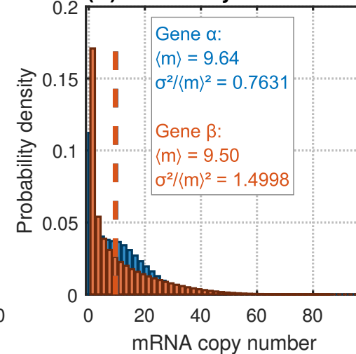
(C) Stationary distribution
