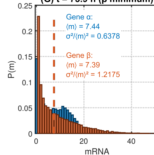
(G) t = 73.9 h ( \beta minimum)
