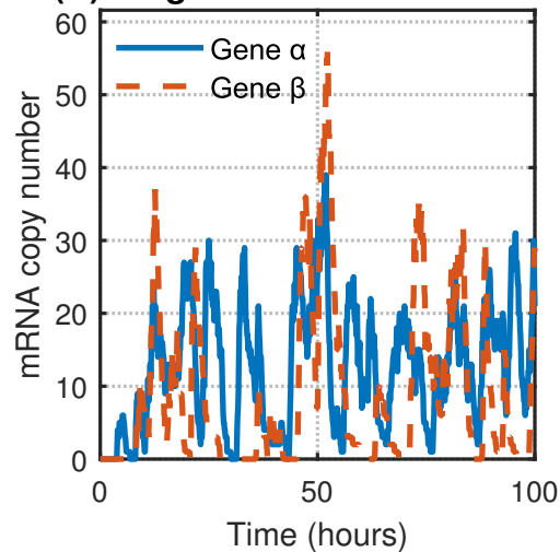
(A) Single stochastic realization
