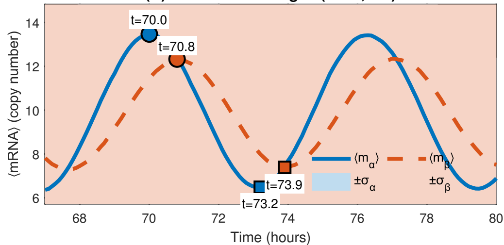
(B) Ensemble averages (n=10,000)
