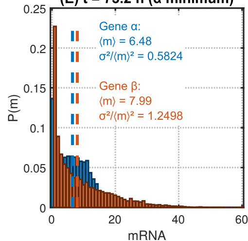
(E) t = 73.2 h ( \alpha minimum)
