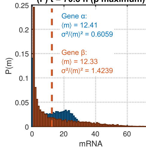
(F) t = 70.8 h ( \beta maximum)
